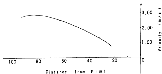
Fig. 3. Average horizontal velocity of pegs in the tunnel floor.
