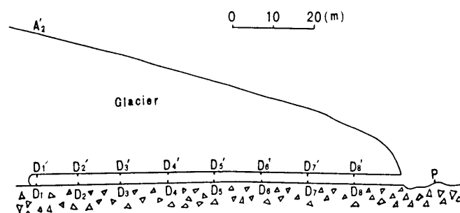
Fig. 2. Longitudinal profile of the ice tunnel 2.
