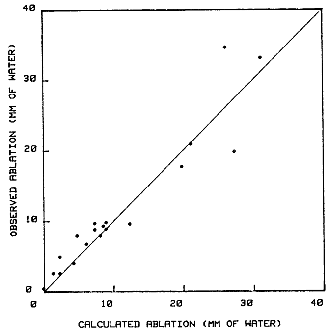
Fig. 5. Plot of total daily observed snowmelt against total daily calculated ablation.
