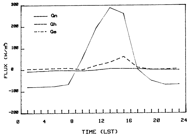
Fig. 2. Diurnal variations of the surface energy balance components on 1 April 1987, under clear conditions (Local Standard Time).
