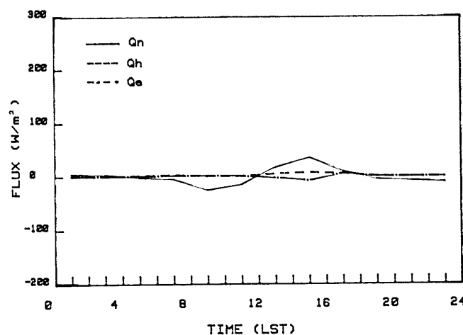
Fig. 3. Diurnal variations of the surface energy balance components on 8 April 1987, under overcast conditions (Local Standard Time).
