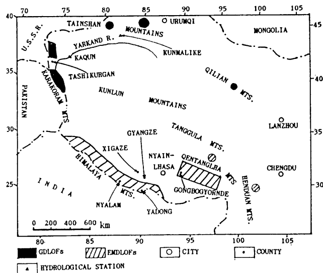
Fig. 1. Distribution of floods from glacier-dammed lakes (GDLOFs) and floods from lakes dammed by end moraines (EMDLOFs).
