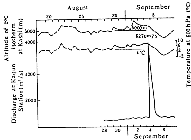
Fig. 3. Hydrograph of the 1961 glacial flood of the Yarkant River (reproduced from Feng and Liu, 1990).
