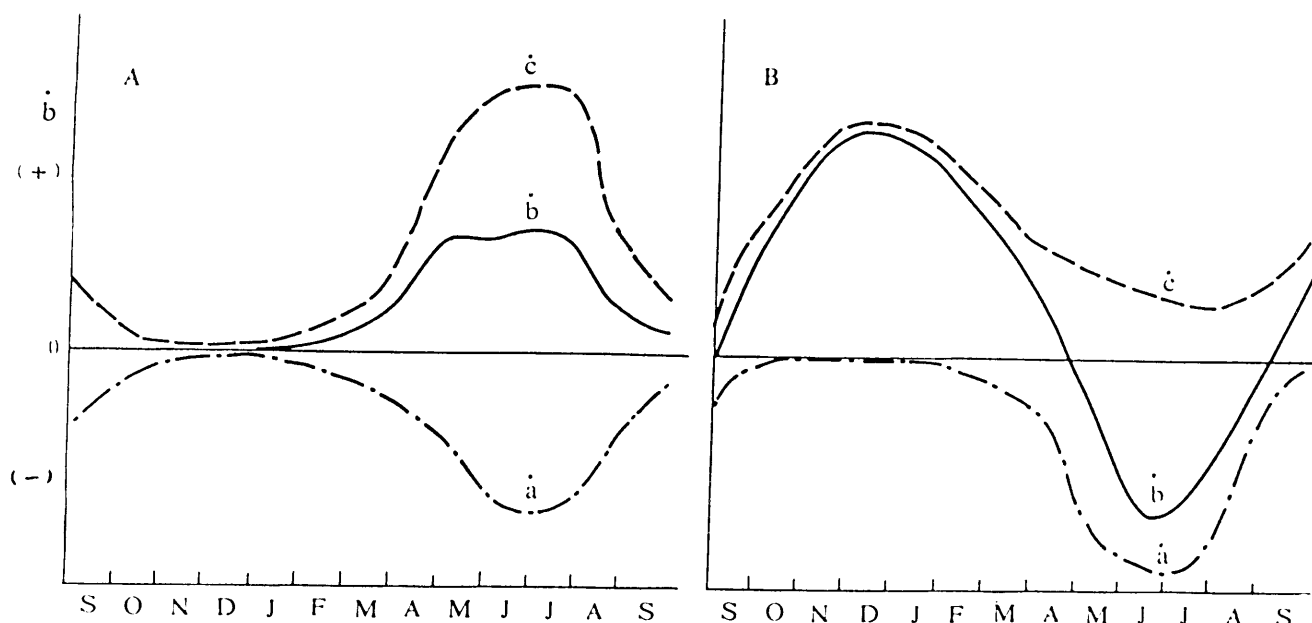
Fig. 1. Illustration of variation of accumulation (c), ablation (a) and net balance (b) for glaciers of the summer-accumulation type (A) and the winter-accumulation type (B) in the accumulation area.
