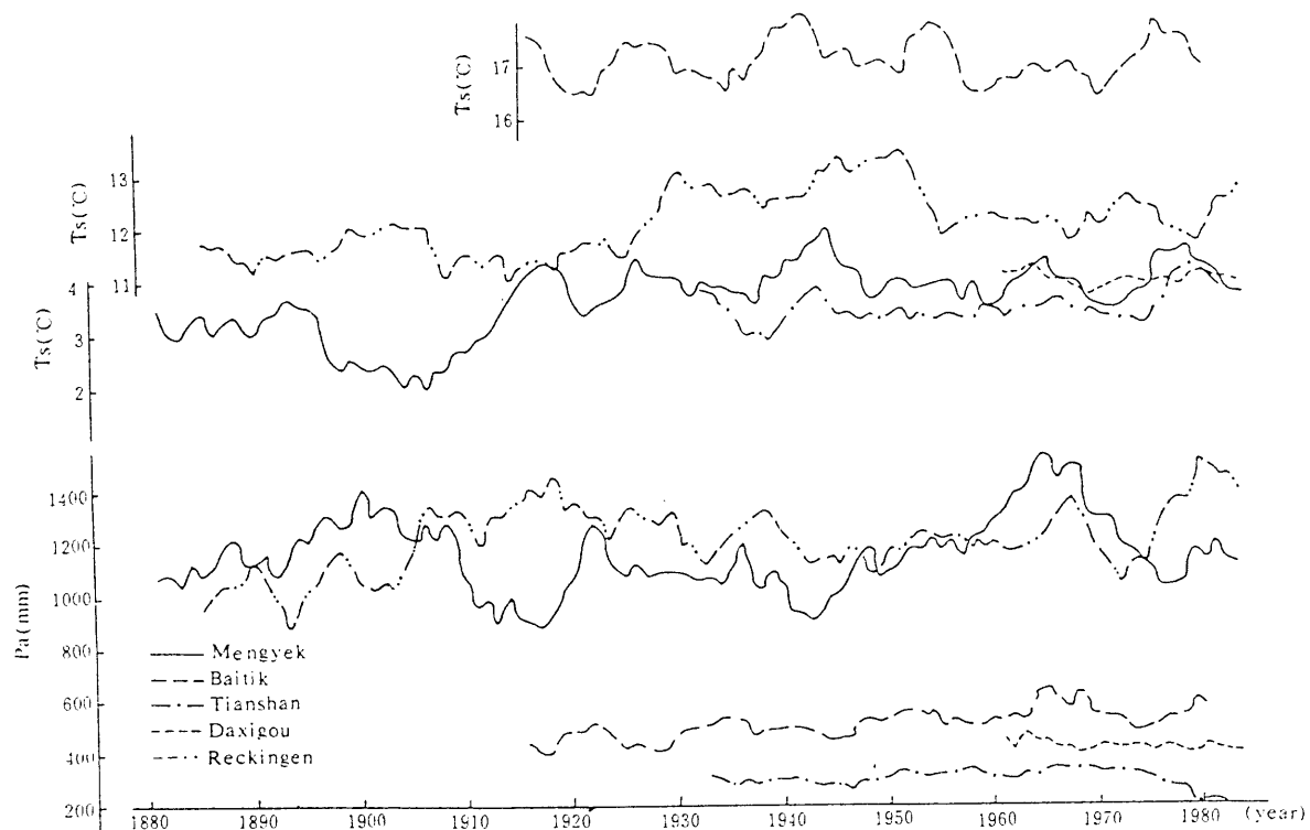
Fig. 3. Five-year moving average curves of annual precipitation ( P_a ) and mean summer temperature ( T_s ) from several meteorological stations in the Tien Shan.
