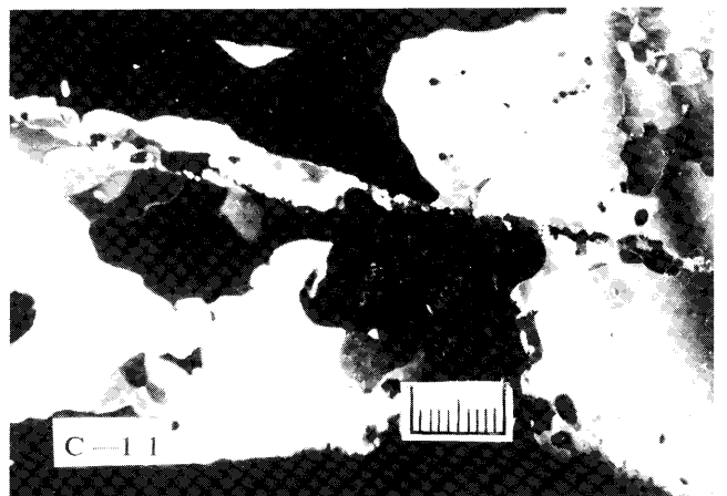
Fig. 5. Photographs of thin sections of ice under cross polaroids showing a possible shear plane (a) and a possible shear band (b) in the ice-laden till bed.
