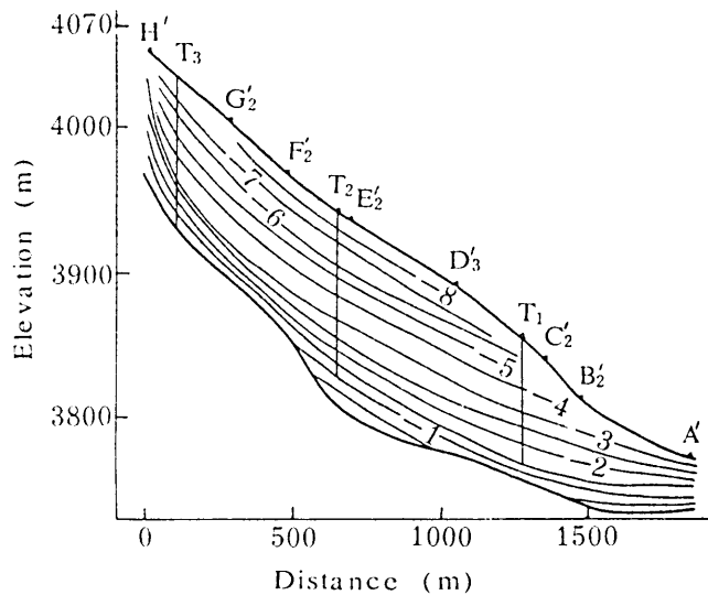
Fig. 2. Modelled two-dimensional temperature profile along the main flowline of the east tributary of Glacier No. 1 (after Cai, 1989).
