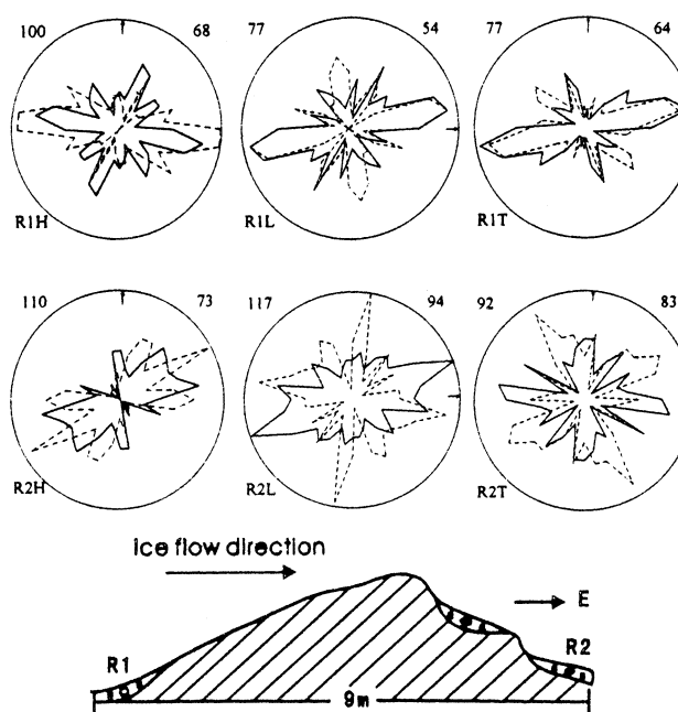
Fig. 5. Cross-section of roche moutonnée from which samples R1 and R2 were collected, and rose diagrams of microfabrics. See Figure 3 for explanation.
