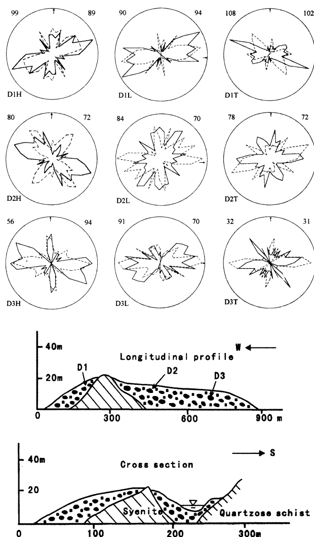
Fig. 7. Longitudinal and transverse cross-sections of drumlin from which samples D1–D3 were collected, and rose diagrams of microfabrics. See Figure 3 for explanation.
