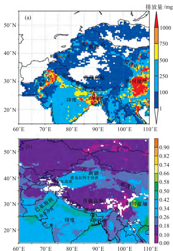
图3 2006年 0.5^{\circ} \times 0.5^{\circ} 东亚、南亚部分地区黑碳排放(a)及2001—2006年该地区大气平均气溶胶光学厚度(b) Fig. 3 0.5^{\circ} \times 0.5^{\circ} BC emission (Mg) of most East and South Asia in 2006 (a) and mean 0.5^{\circ} \times 0.5^{\circ} AOD of East and South Asia during 2001–2006 (b)
