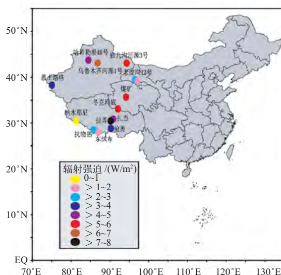
图4 中国西部冰川表面雪中黑碳辐射强迫 Fig. 4 Distribution of radiative forcing of BC deposits in the surface snow of the glaciers in west China
