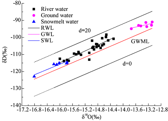
Figure 4. Relation between \delta^{18}\text{O} and \delta\text{D} and deuterium excess values distribution during the spring flood period in Yushugou River basin.
